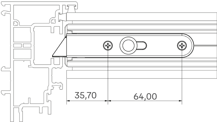
Slot position on lower sash interlock for Tilt Latch (fixing holes as upper sash)
