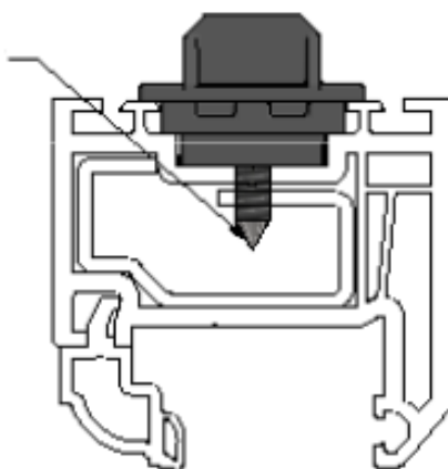
Typical application requiring Spacer
