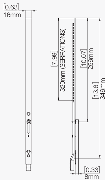
SPL2480R-104 Roller Extension, Brushed SS304
