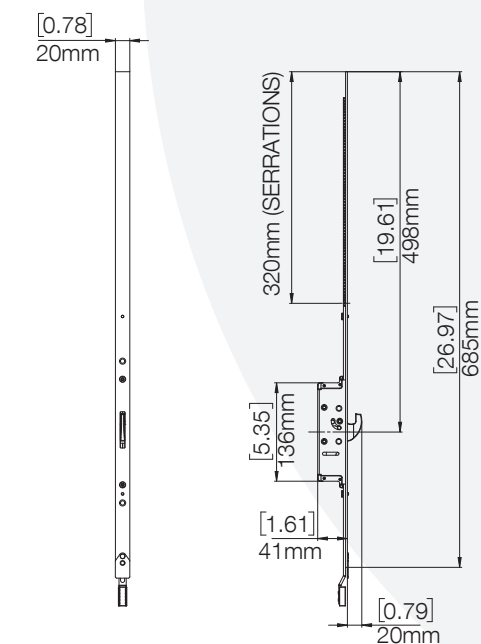
SPL2481HK-104 Hook Extension, Brushed SS304
