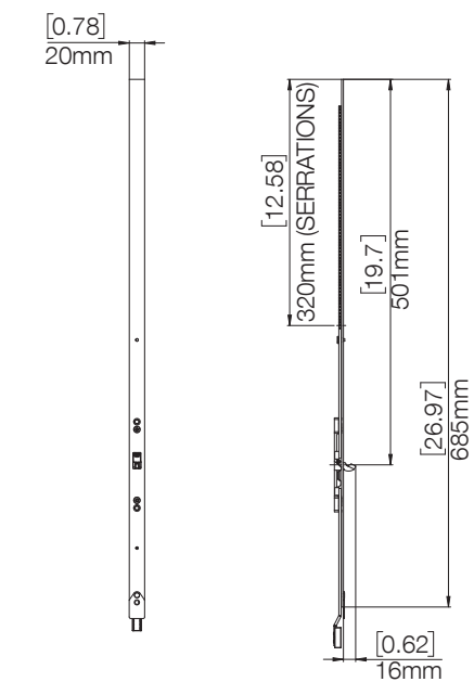
SPL2481TG-104 Tongue Extension, Brushed SS304
