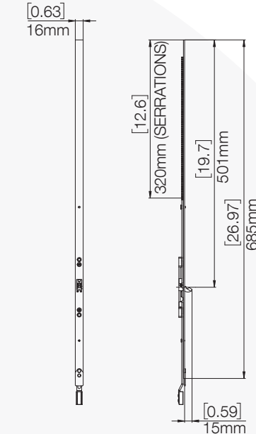
SPL2480TG-104 Tongue Extension, Brushed SS304
