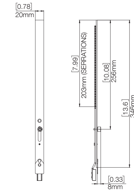
SPL2481R-104 Roller Extension, Brushed SS304
