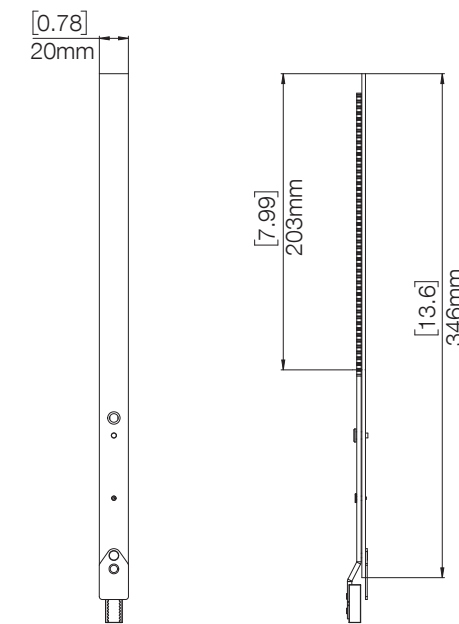
SPL2481-104 Stud Extension, Brushed SS304
