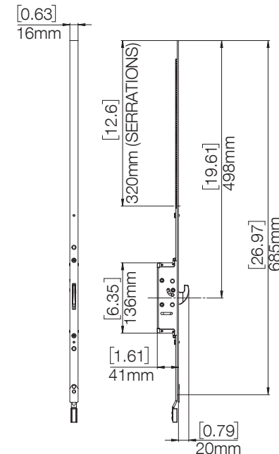
SPL2480HK-104 Hook Extension, Brushed SS304
