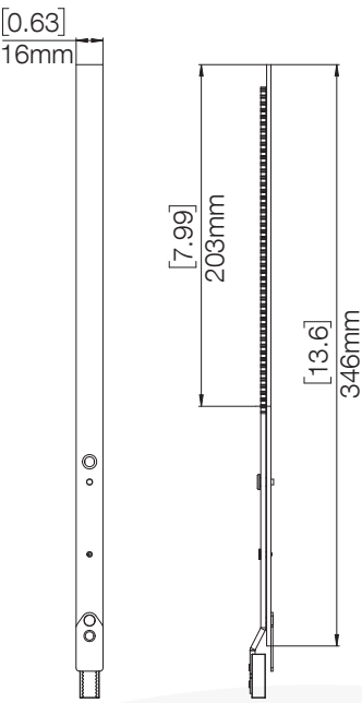
SPL2480-104 Stud Extension, Brushed SS304
